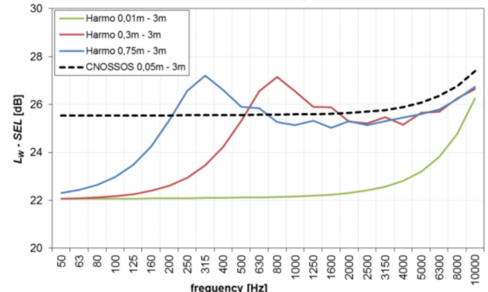
Transfer functions from L_W to SEL
